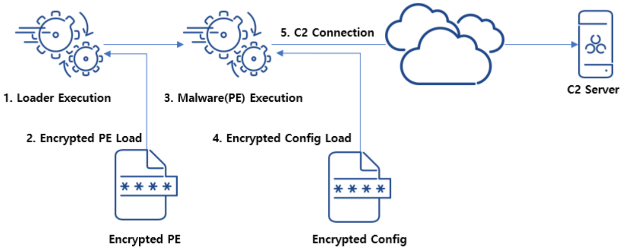
Figure. Backdoor operation process
